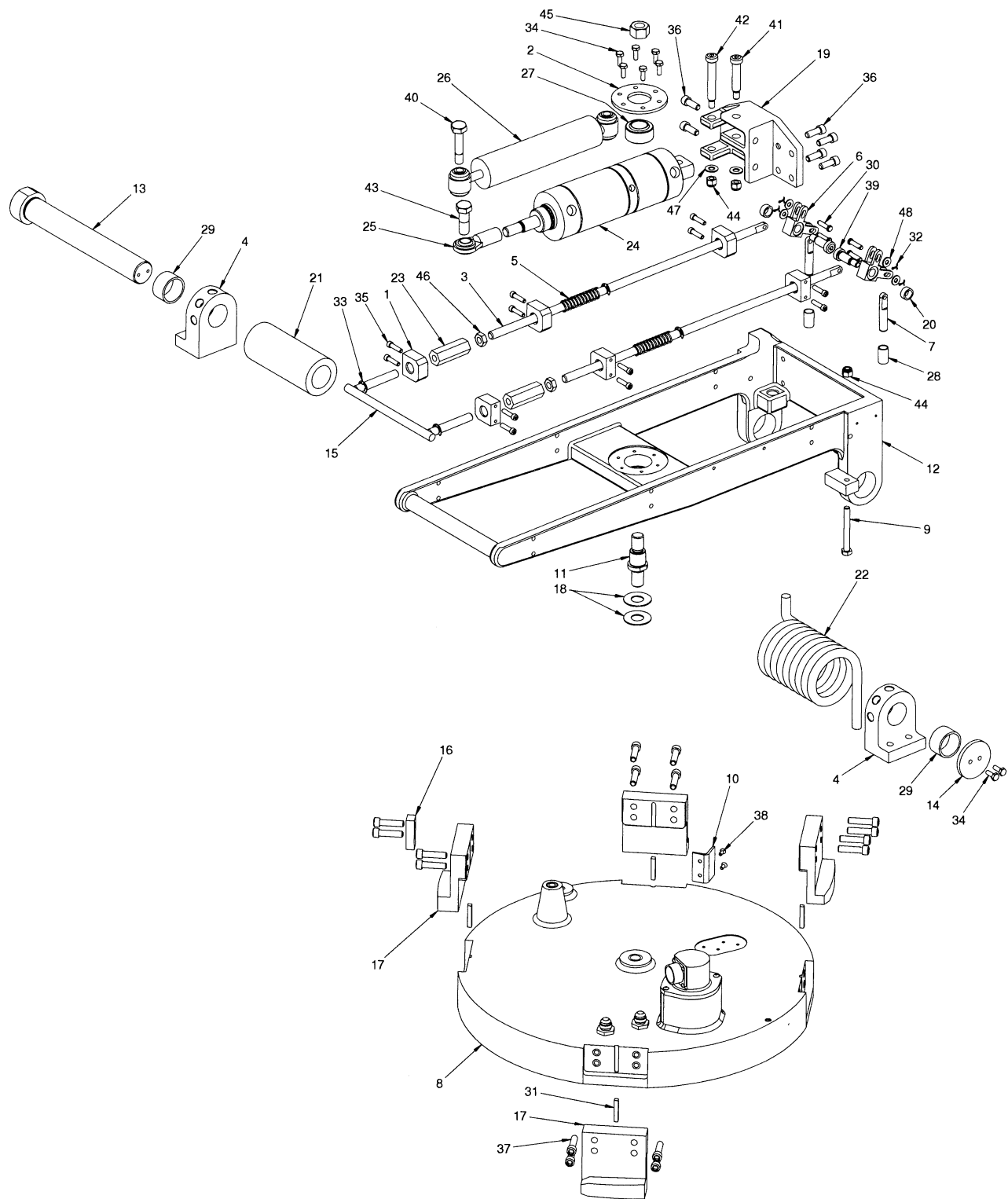
Figure 3. CMU Door Assembly.
