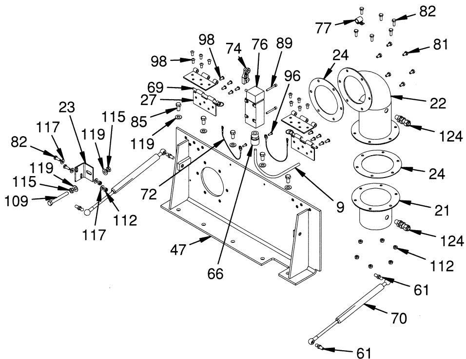
Figure 2B. CMU Safety Cover Bracket Subassembly.
